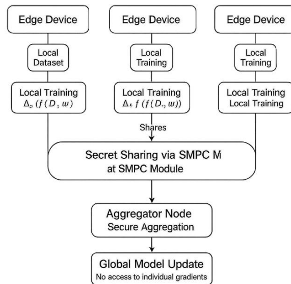
Figure 4. Secure Federated Optimization Workflow Using SMPC in IIoT
