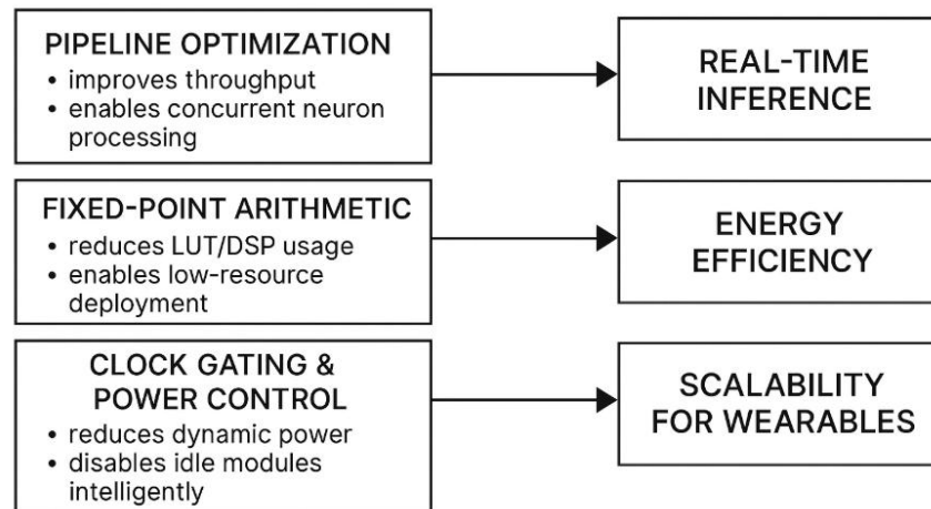
Figure 4. Optimization Strategies for SNN Accelerator Design
