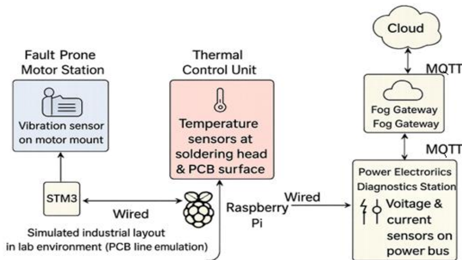
Figure 5. Simulated Industrial Testbed for SSN Evaluation in PCB Assembly Line
