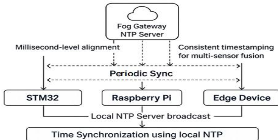
Figure 4. Time Synchronization Mechanism Using Local NTP Server in SSN
