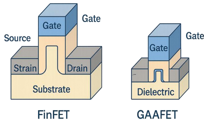
Figure 6. Cross-Sectional Comparison of FinFET and GAAFET Architectures
