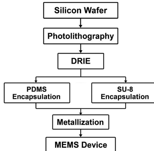
Figure 2. Fabrication Workflow Diagram for visual representation
