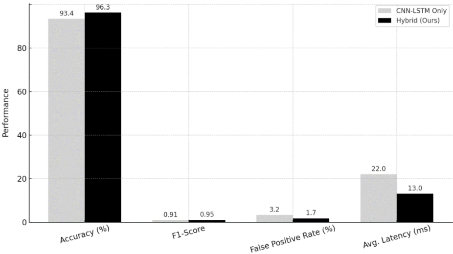
Figure 5. Performance Comparison of CNN-LSTM Only vs. Hybrid Model
